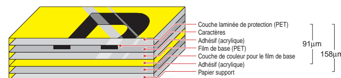
STRUCTURE DU RUBAN LAMINE BREVETE BROTHER
